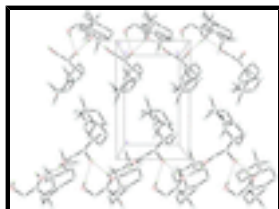
Fig. 2. A packing diagram of the title compound viewed along the c axis, showing screw chains running along the [0\ 1\ 0] direction. For clarity, H atoms not involved in hydrogen bonds were omitted. Hydrogen bonds are shown as dashed lines.
